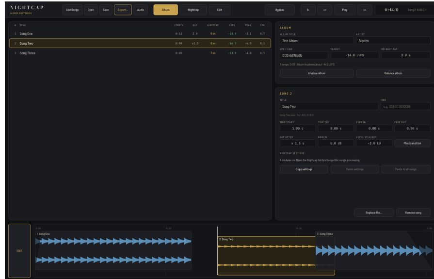
The Album view: songs on the left, the album and the selected song on the right, the timeline along the bottom.
